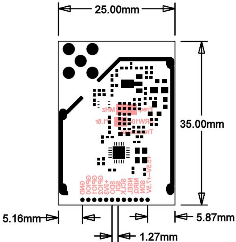
DIP Package V1.6
